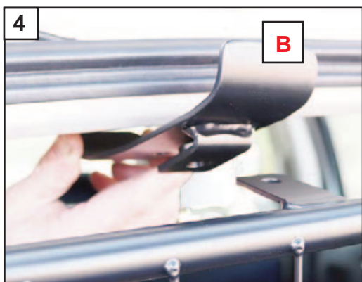
4 From inside the car insert bracket B
